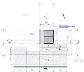
A103- N01-Simple 1:50
