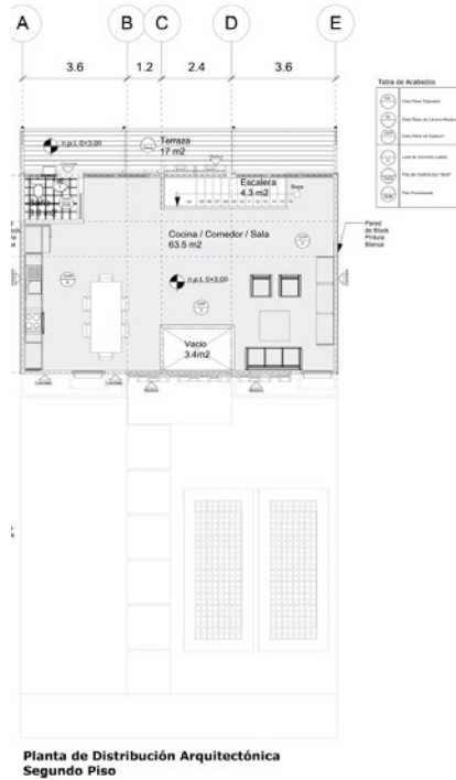
Floor Plan_Level 2
